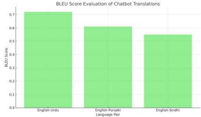
Figure 4: BLEU Score Evaluation of Chatbot Translations
